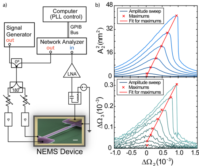
Figure 2. (a) Circuit diagram for measurement of intermodal nonlinearities in doubly clamped PZE-actuated/PZM-sensed beam; intramodal nonlinearities are measured without using this circuit; see Figure 1a. A signal generator is used to excite the device at a range of frequencies around the resonance of mode q , while the frequency of mode p is measured using a network analyzer with a digital PLL. (b) Example measurement of intra- and intermodal nonlinearities. Data in the upper graph is due to the intramodal nonlinearity of the second mode. Data in the bottom graph shows the effect of intermodal nonlinearity on the frequency shift of the third mode due to excitation of the second mode. Comparing these two data sets enables the intermodal nonlinearity coefficient to be extracted.
