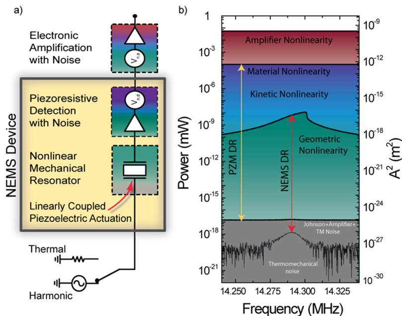
Figure 1. (a) Schematic of measurement design and protocol. When the switch is set to “Thermal”, the device is passively excited by thermal fluctuations. The resulting mechanical motion is transduced into electronic signals via the piezoresistive detector, which can be amplified through use of an external electronic amplifier. Other sources of noise from the detection and amplification exist. Setting the switch to “Harmonic” actively excites the device enabling interrogation of nonlinear response. (b) Illustration of relevant system dynamic ranges. The thermomechanical noise (bottom of red arrow) is extracted from the total noise spectrum (bottom of yellow arrow) and used to calibrate the right-hand vertical axis within the dynamic range (DR) of the metallic piezoresistor (PZM). The upper limit of the DR of the NEMS device is defined by the nonlinear critical amplitude and clearly resides within PZM DR. This enables measurement of the nonlinear properties of the device.
